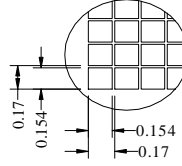
Detail "A" Scale (10:1)
